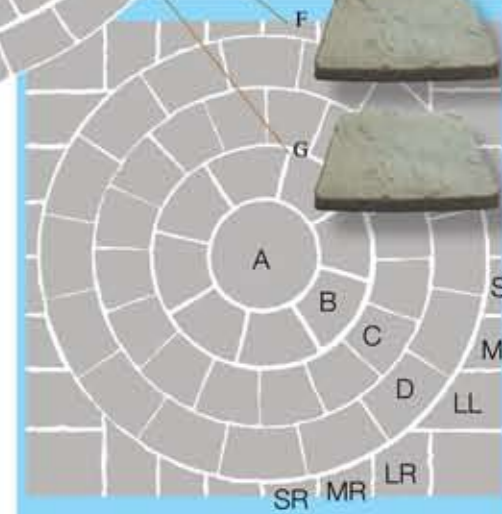
Classic Rotarea & Squaring off Kit Project Pack 3.66m (12') diameter circle squared off to 3.96m sq coverage 15.68 sq m - 69 pieces - 1452kg
