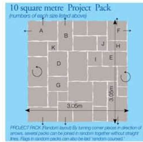
PROJECT PACK (Random layout) By turning corner pieces in direction of arrows, several packs can be joined in random together without straight lines. Flags in random packs can also be laid 'random coursed'.
