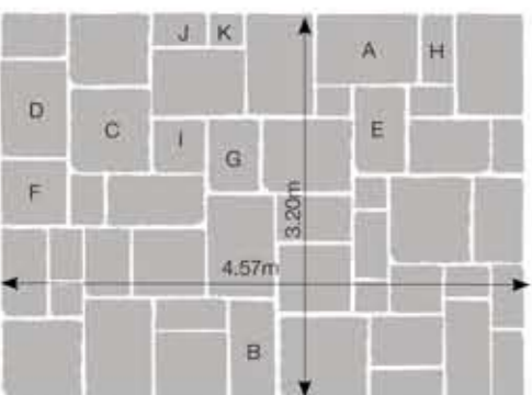
Random Flags (use approximately equal numbers of each size)
